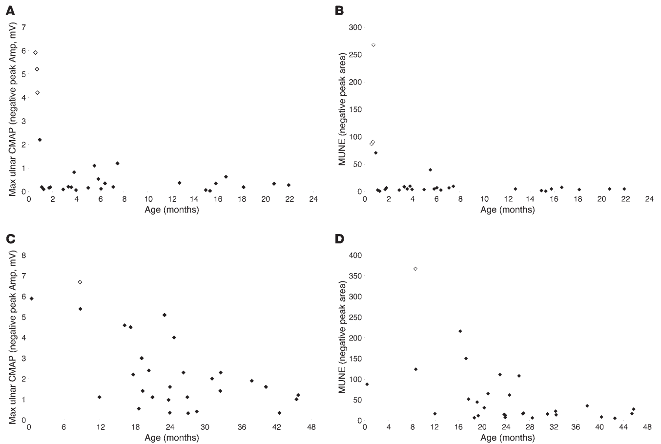
Figure 1 Denervation status in relation to age in SMA type I and SMA type II. (A) Maximum ulnar CMAP amplitude and (B) MUNE values versus age in SMA type I infants, birth to 24 months. (C) Maximum ulnar CMAP amplitude and (D) MUNE values versus age in SMA type II children from birth to 48 months of age. For all panels, white diamonds indicate presymptomatic infants (identified via genetic testing due to an affected sibling). Black diamonds indicate already symptomatic infants. Adapted with permission from Annals of Neurology (Figures 2 and 3; ref. 20).
